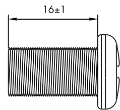
M5*16 Screw (zinc plating)
