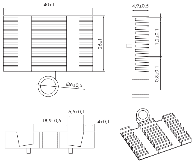
12 core splicing holder 40 mm, crimping type
